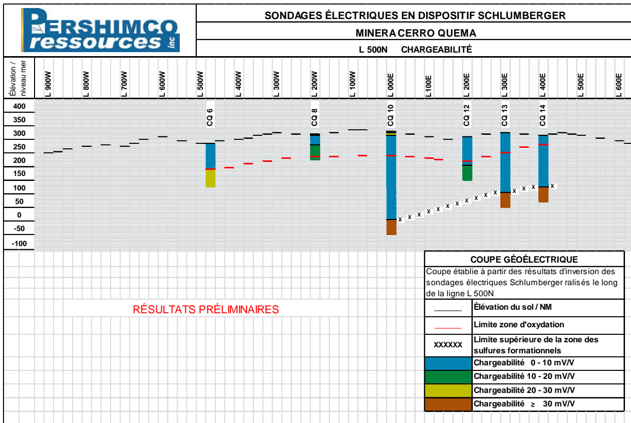
Figure 2 TL 5+00N, Preliminary Inversion on Shlumberger Essays
