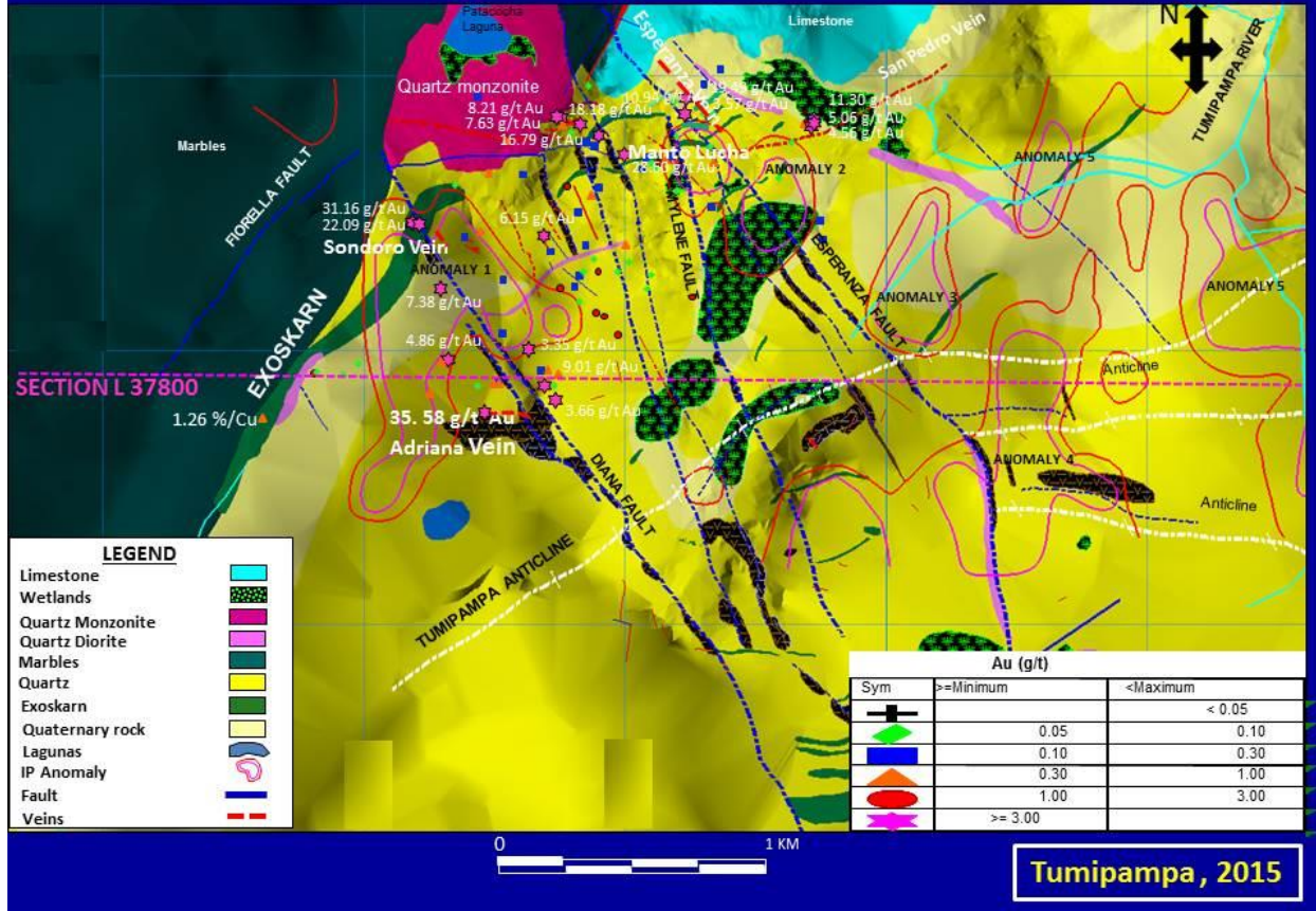
Figure 1. Geological Map of the Disseminated Gold Zone at Tumipampa
