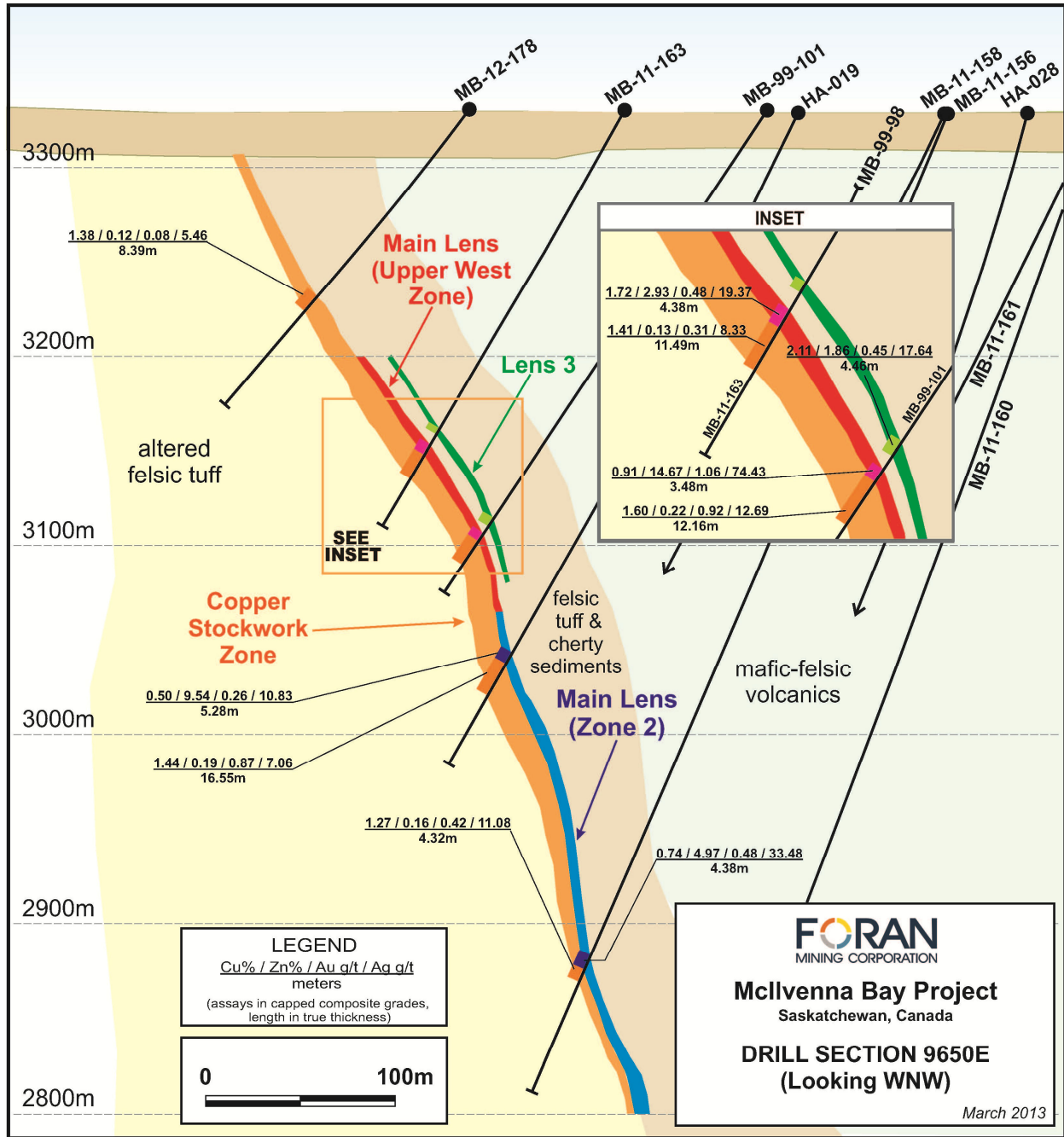
Figure 1. Representative cross section through the Deposit.
