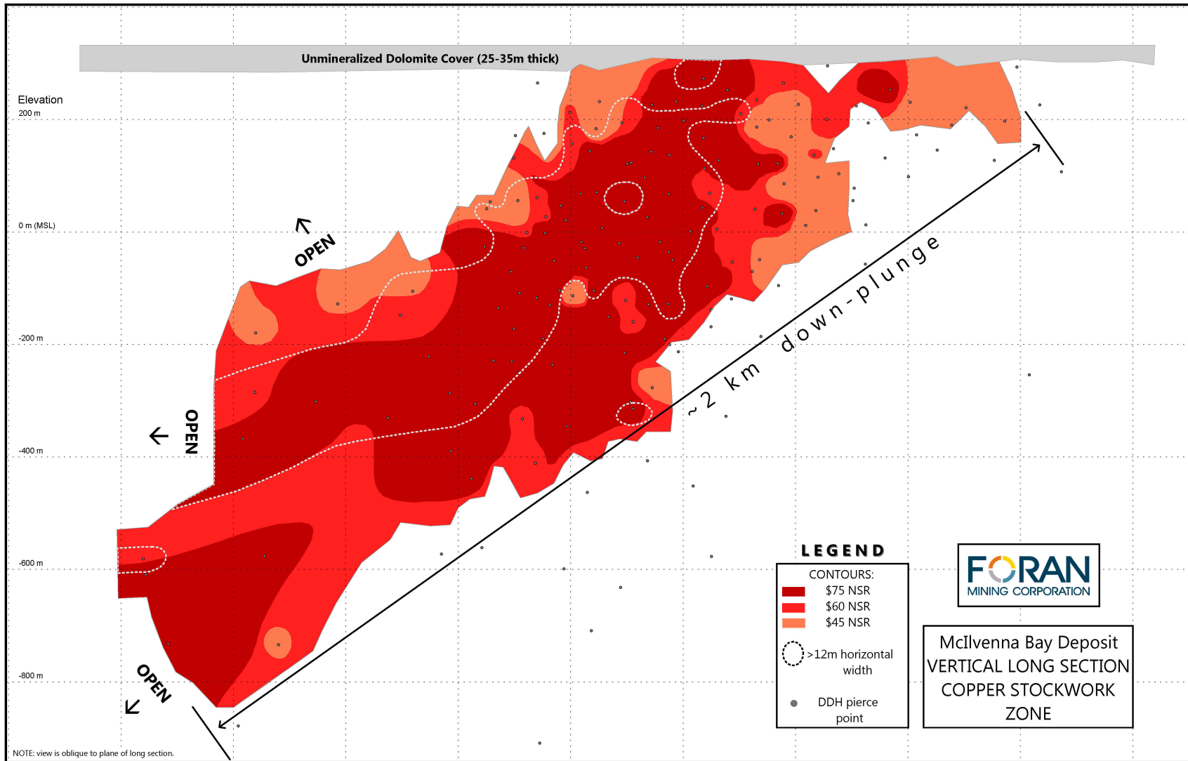
Figure 2. Longitudinal Section for the Copper Stockwork Zone.
