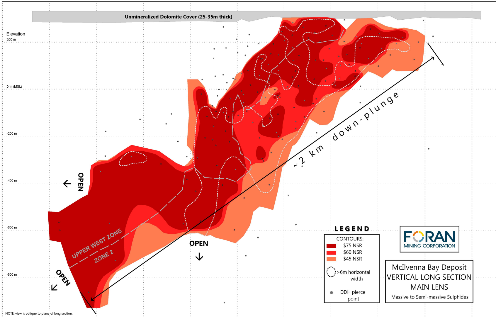
Figure 3. Longitudinal Section for the Main Lens (Upper West Zone and Zone 2).
