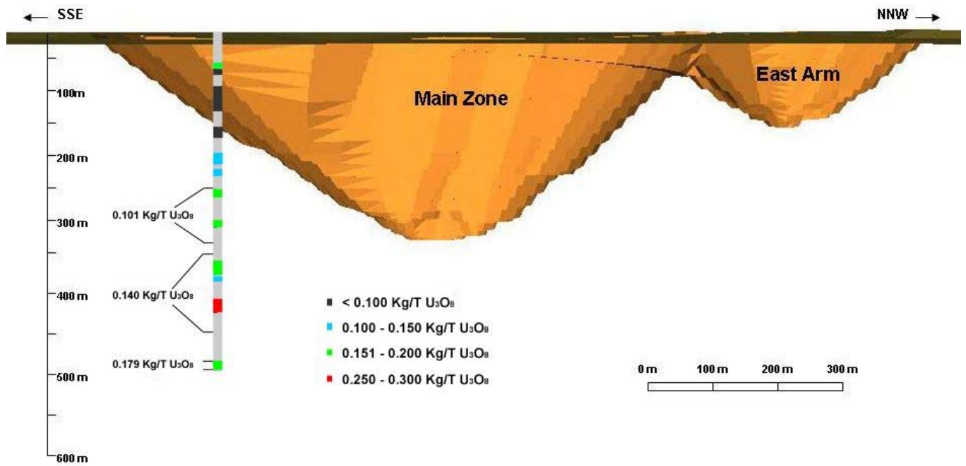
Figure 1 – NE-SW Schematic Longitudinal Section of Proposed Valencia Pit Looking West
