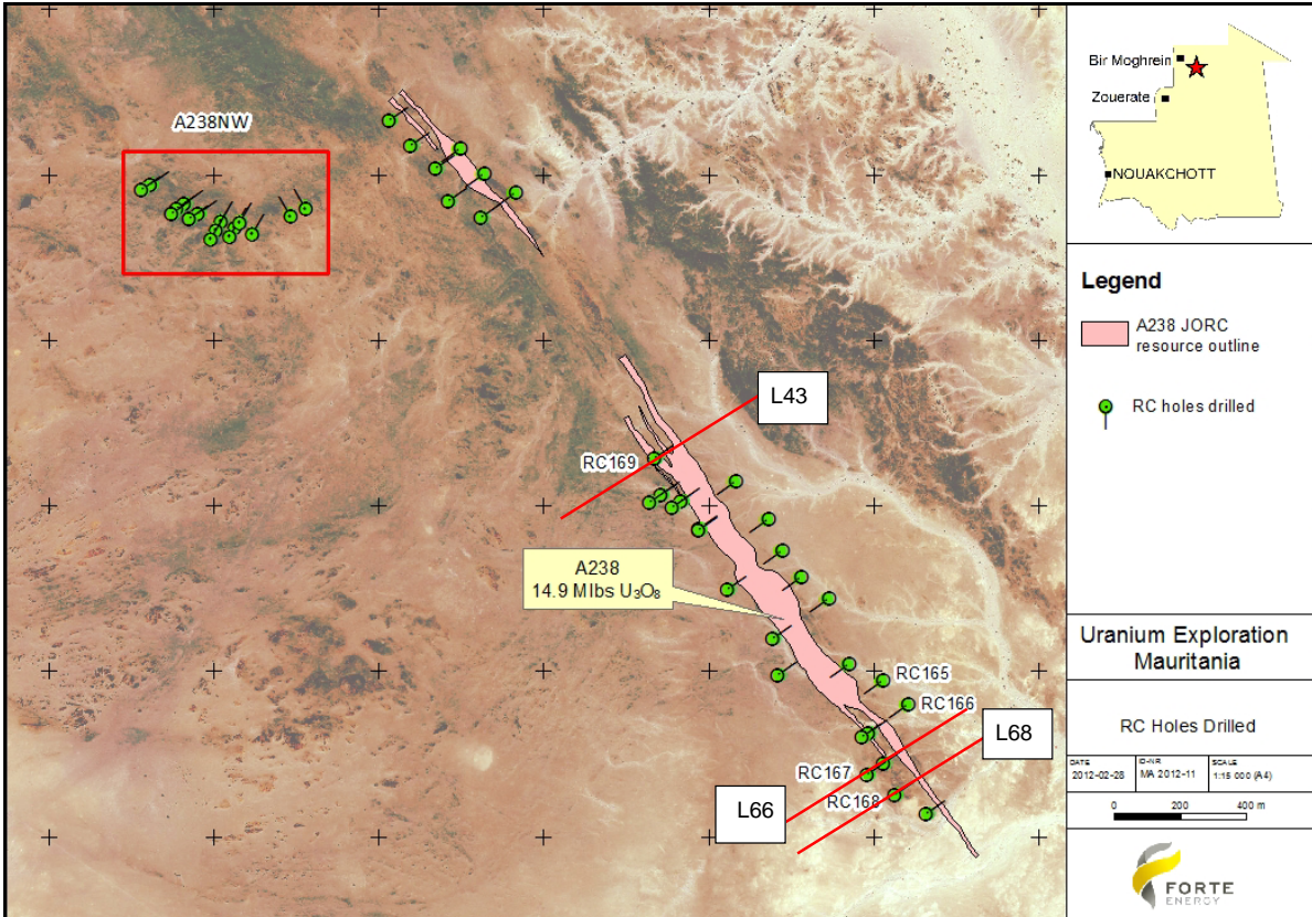
Figure 1: A238 Drilling
