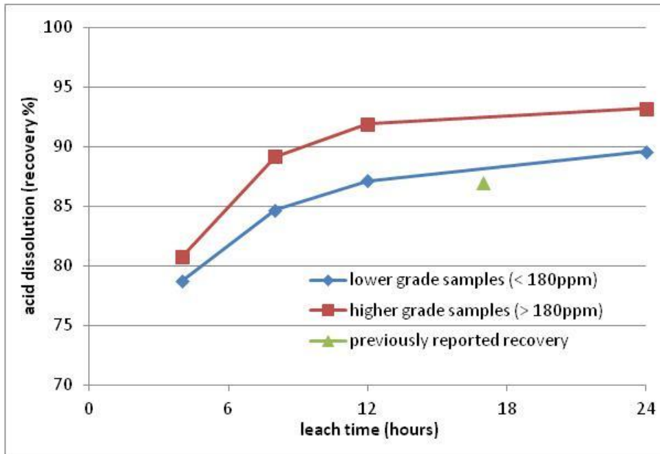
FIGURE 6. Leach recovery performance comparing higher grade with lower grade samples (weighted average for both data sets).
