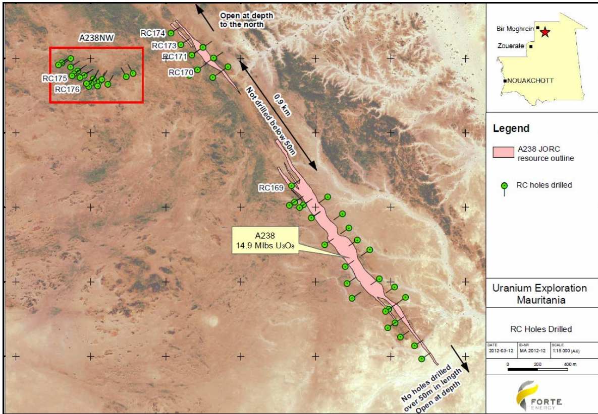
Figure 1: A238 Drilling
