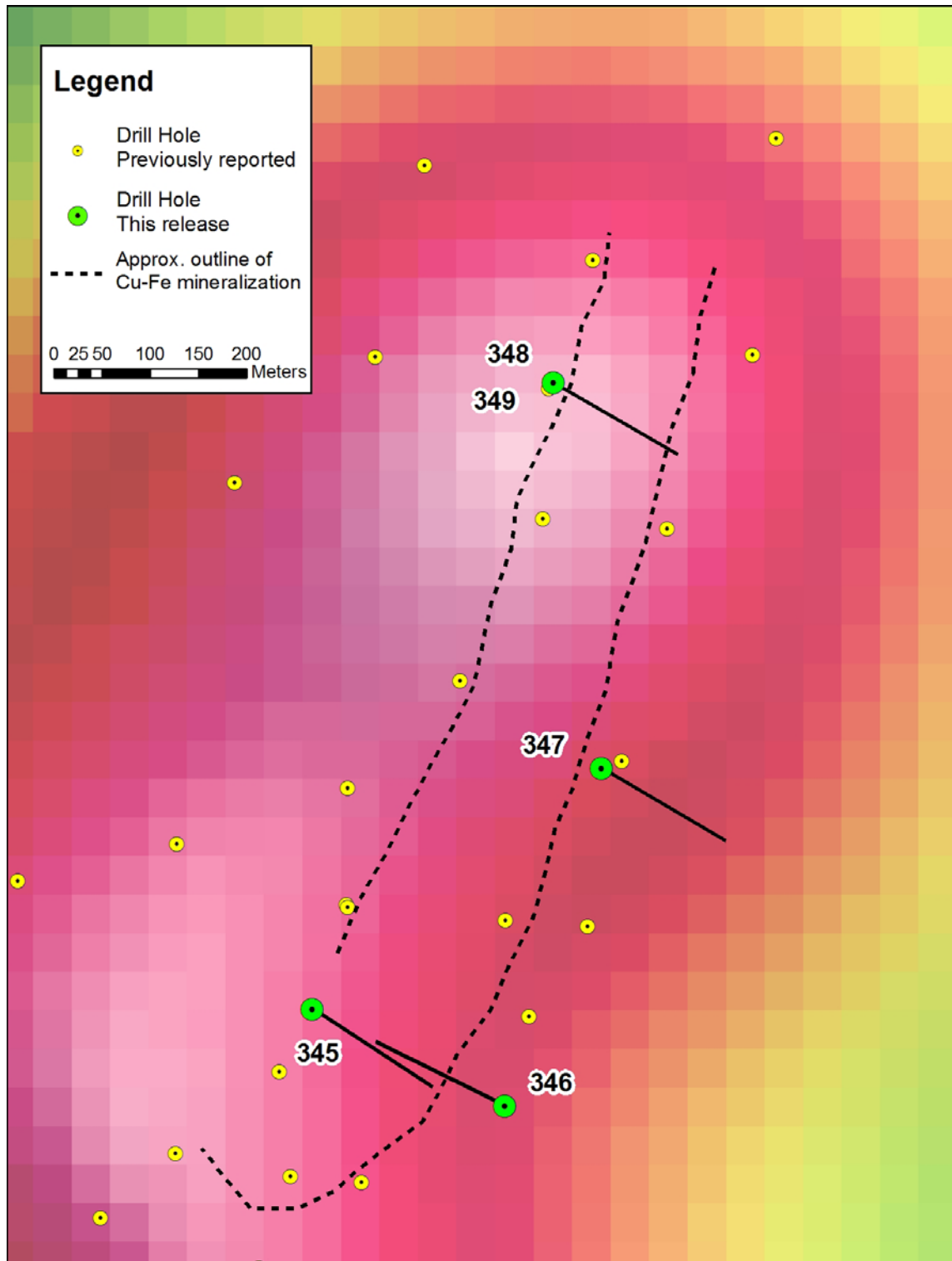
Figure 1: FALCON TEM gravity image showing the Iris Norte zone. The mineralized zone is approximately 100-200m wide with a strike length of approximately 1,000m. The deposit remains open at the centre of the gravity anomaly to the southwest and to the north. Drill holes are widely spaced.
