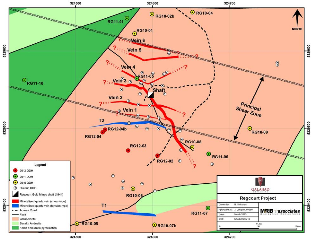
Figure 1: Drill-holes and projected surface traces of principal veins at the Regcourt Project.
