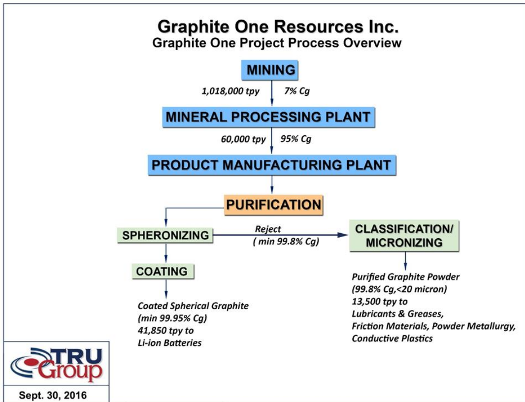
Figure 2: Graphite One Project Mining & Process Overview
