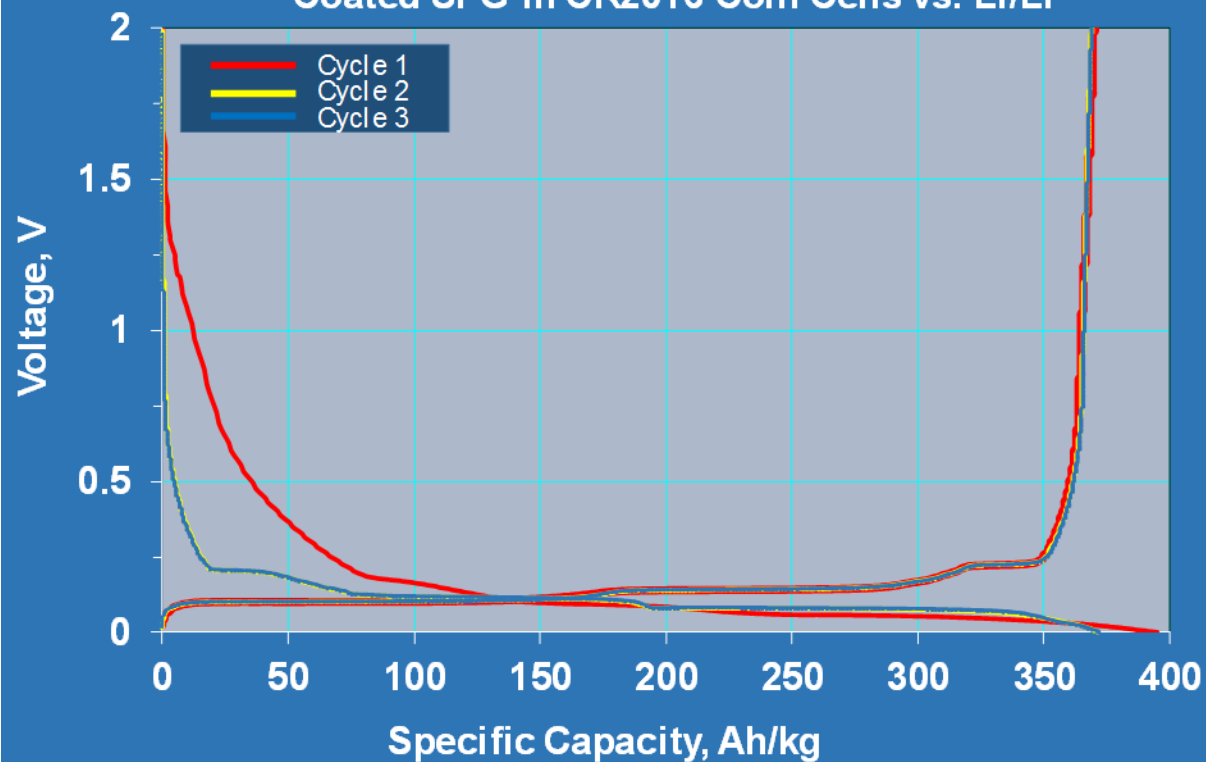
Figure 2: Initial Galvanostatic Cycling of Graphite One Coated SPG in CR2016 Coin Cells vs. Li/Li +
