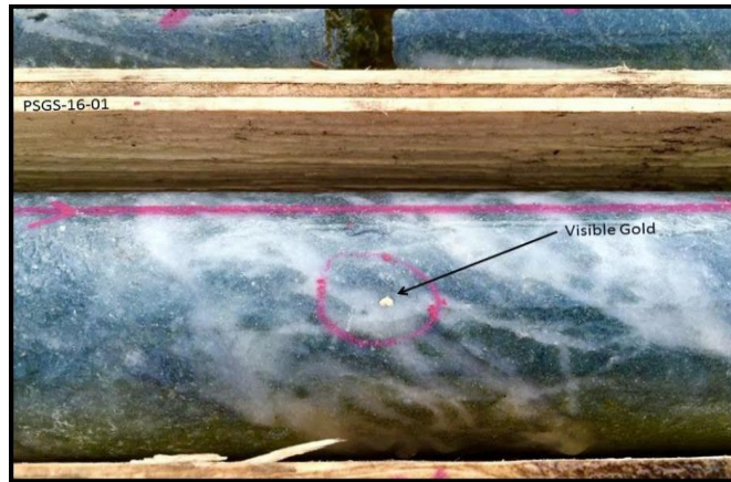
PSGS16-01 Native gold in upper stockwork zone
