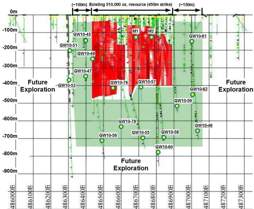
Figure 1. Longitudinal Section - Frankfield East Gold Deposit (2010 Drill Program Update)
