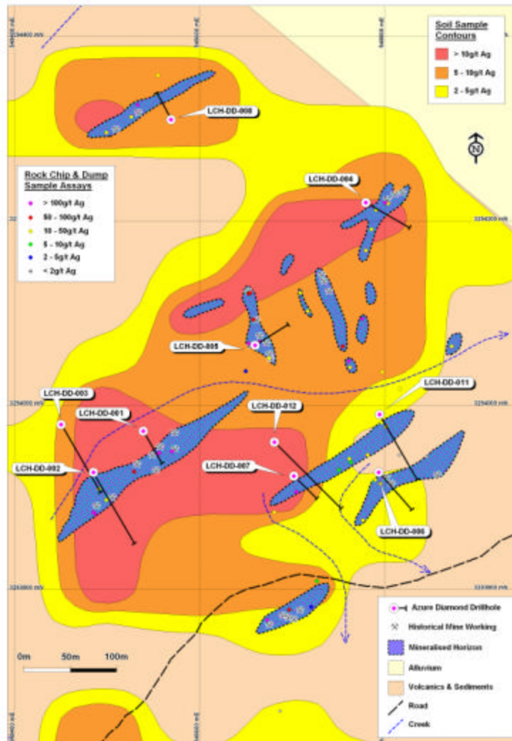
Figure 1. Los Chinos drill hole locations, interpretive geology, and soil sampling contours (source: Azure Minerals Ltd).
