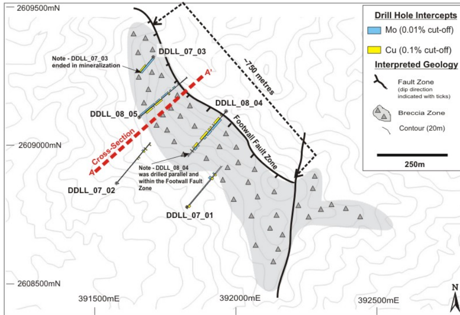
Figure 1. Los Laureles drill holes with interpretative geology.
