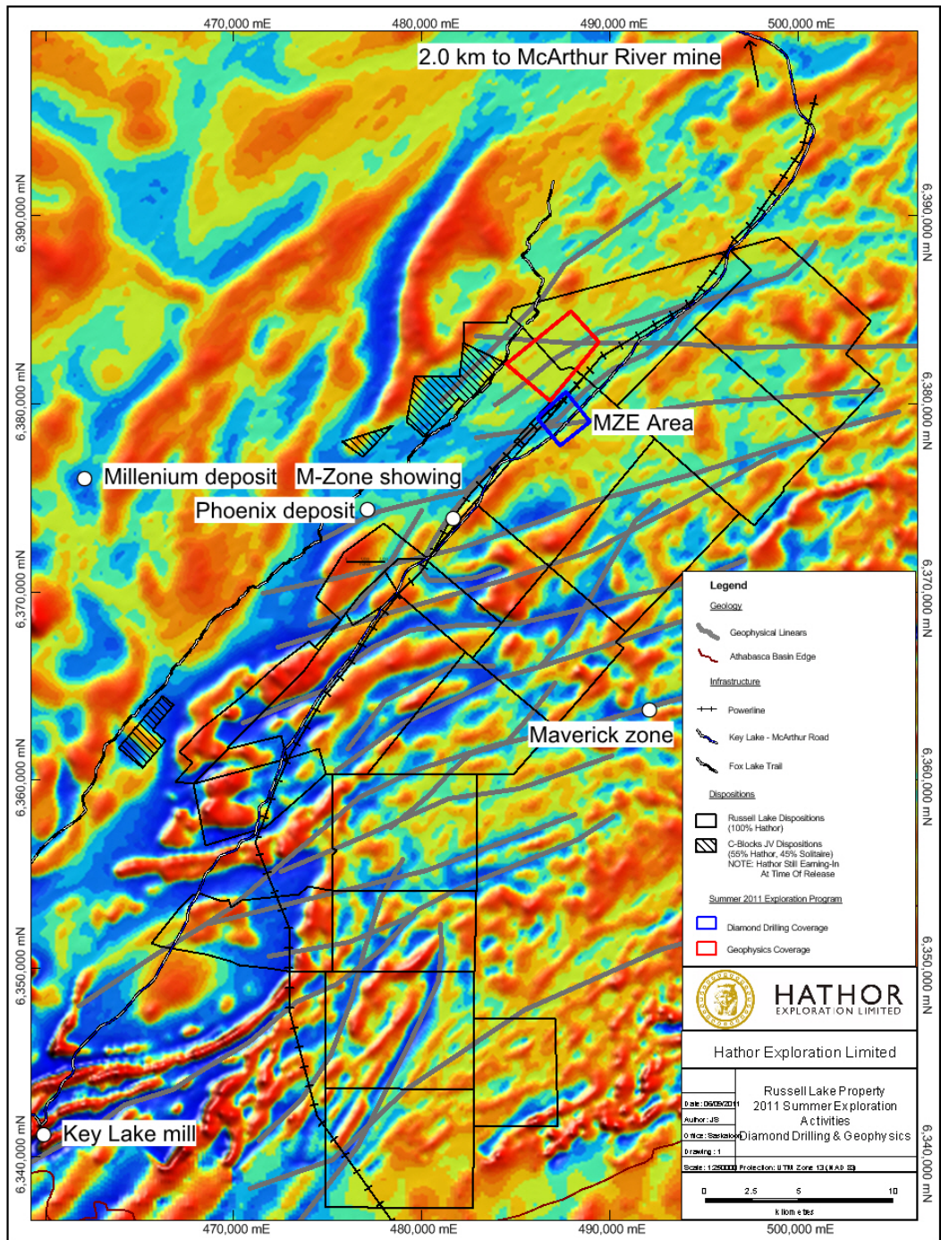
Figure 2. Airborne magnetic map of the southeastern part of the Athabasca Basin (from Saskatchewan Energy and Mines). Thin solid black line outlines Russell Lake Property. Thick grey lines are major structural trends. The MZE target area is highlighted.
