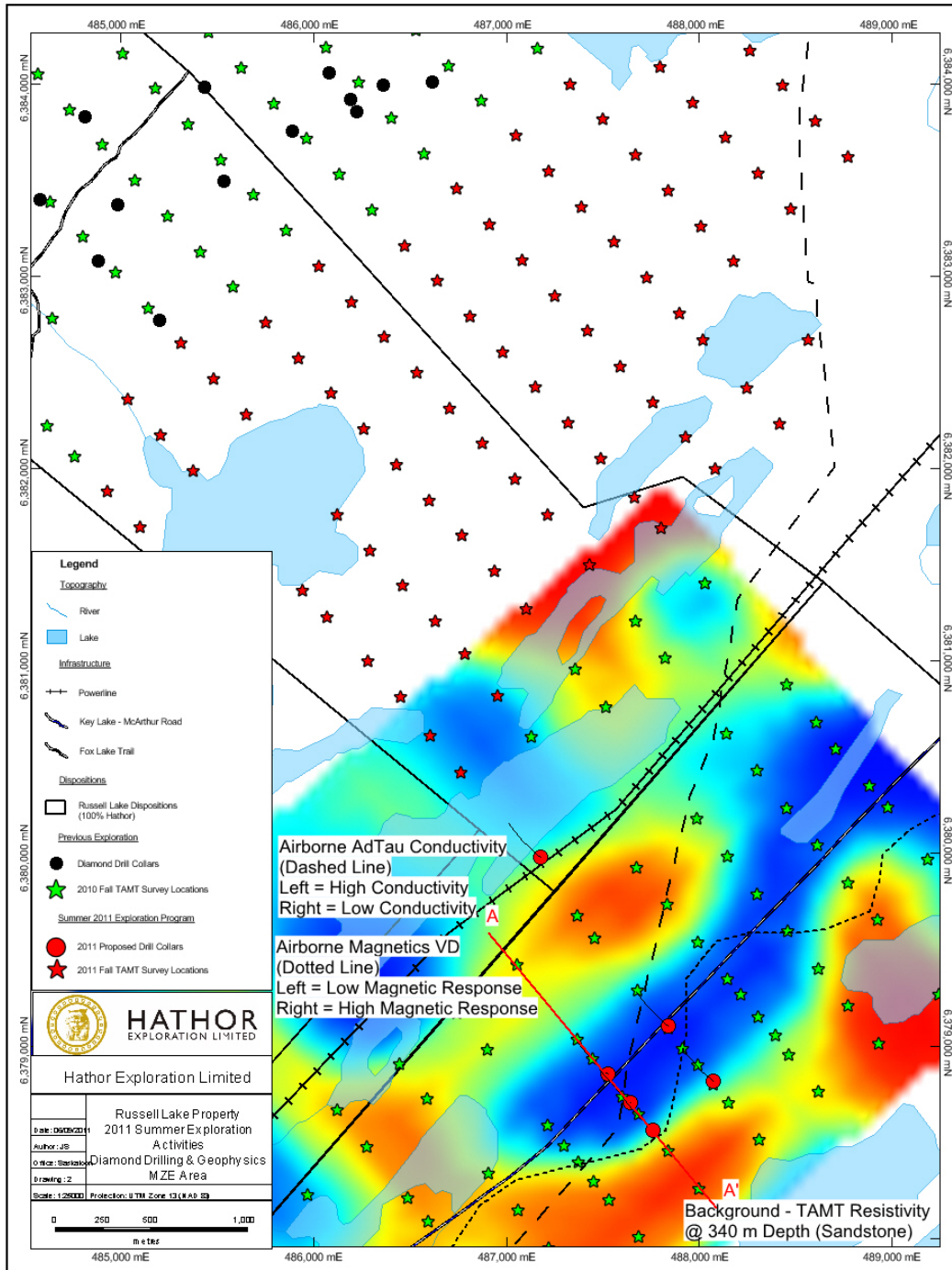
Figure 4. Plan map of the MZE target area showing the location of the planned drill holes and completed AMT surveys. The background is the 340 m depth slice of 2010 AMT survey.
