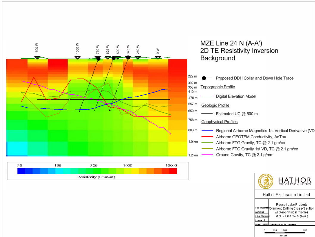
Figure 5. AMT pseudo-section showing the planned drill fence at MZE. Various geophysical profiles are also shown to highlight the integration of gravity, EM and magnetic anomalies.
