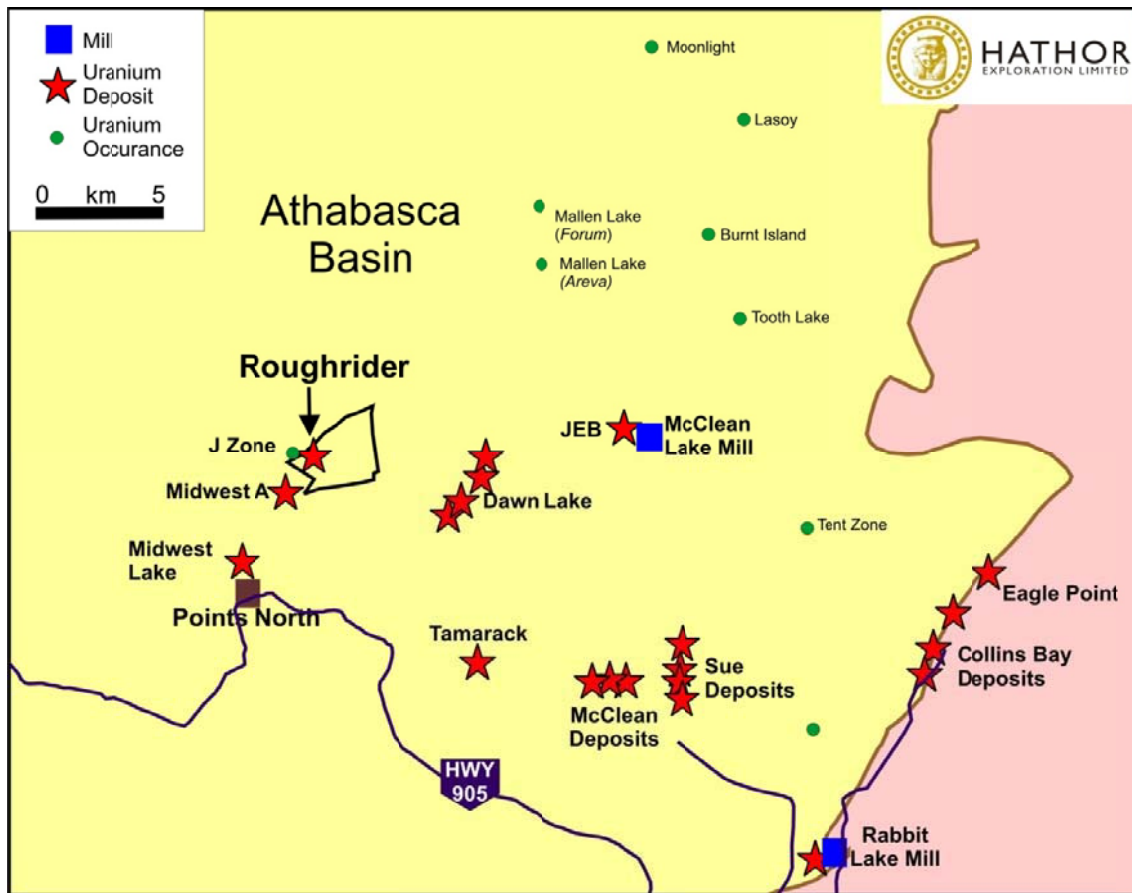
Figure 1. Location map for Roughrider uranium deposit, northeastern Athabasca Basin, Saskatchewan.
