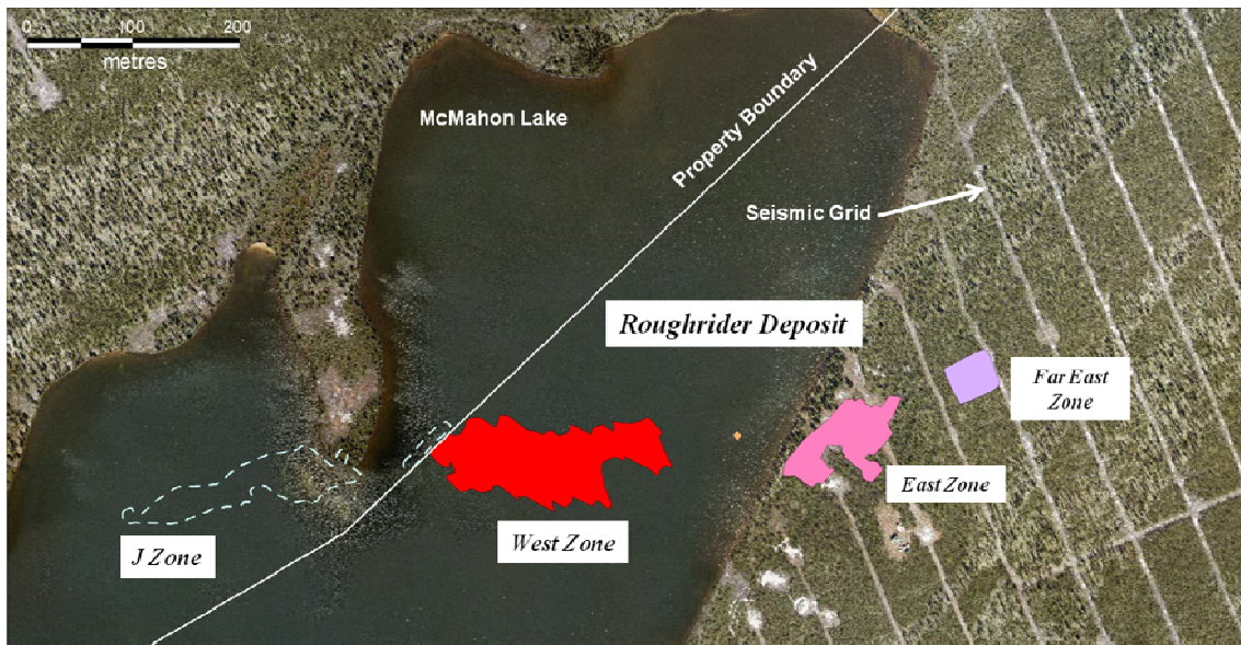
Figure 3. Aerial view of Roughrider uranium deposit. Outline of West Zone is from recent NI43-101 report (Keller et al. 2011). Outline of East Zone encompasses 2010 drill holes with uranium mineralization between L 100 W and 20 E (120 m strike). Outline of J-Zone is schematic and is from website of Fission Energy.
