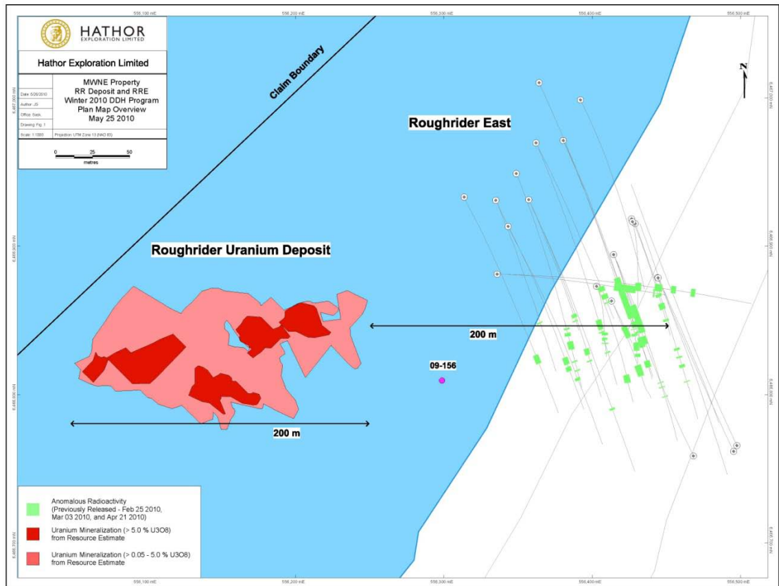
Figure 1. Plan map showing Roughrider Uranium Deposit and Roughrider East discovery.
