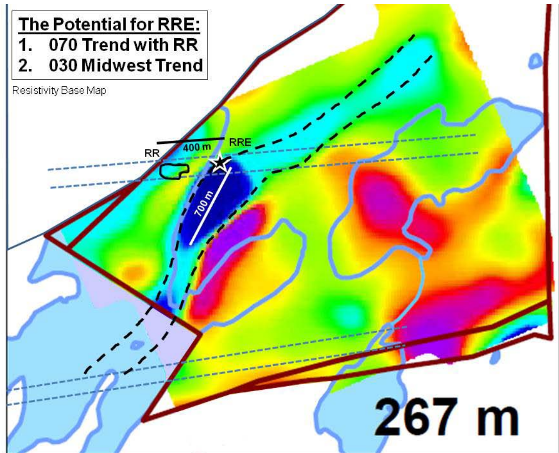
Figure 6. Integrated exploration target for Roughrider East, where mineralization is open to the south-southwest along the Midwest trend as defined by resistivity data. Base map projects resistivity data at a 267 metre depth slice.
