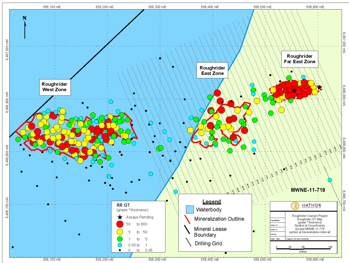
Figure 1: Plan map of Roughridger Uranium Deposit with unconformity pierce-points of drill holes colour-coded based on GT value. Outline of West and East Zones are from recent NI 43-101 report (Keller et al. 2011). The surface projection of the mineralization in drill hole MNWNE-11-719, to the southeast of the Far East Zone, is shown.
