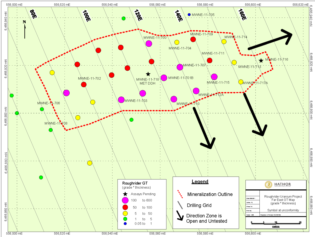
Figure 2: Grid line plan map of Far East Zone at Roughrider Uranium Deposit, with drill holes completed during 2011 winter (unlabelled) and summer (labelled) drill programs. Drill holes are colour-coded based on GT value.
