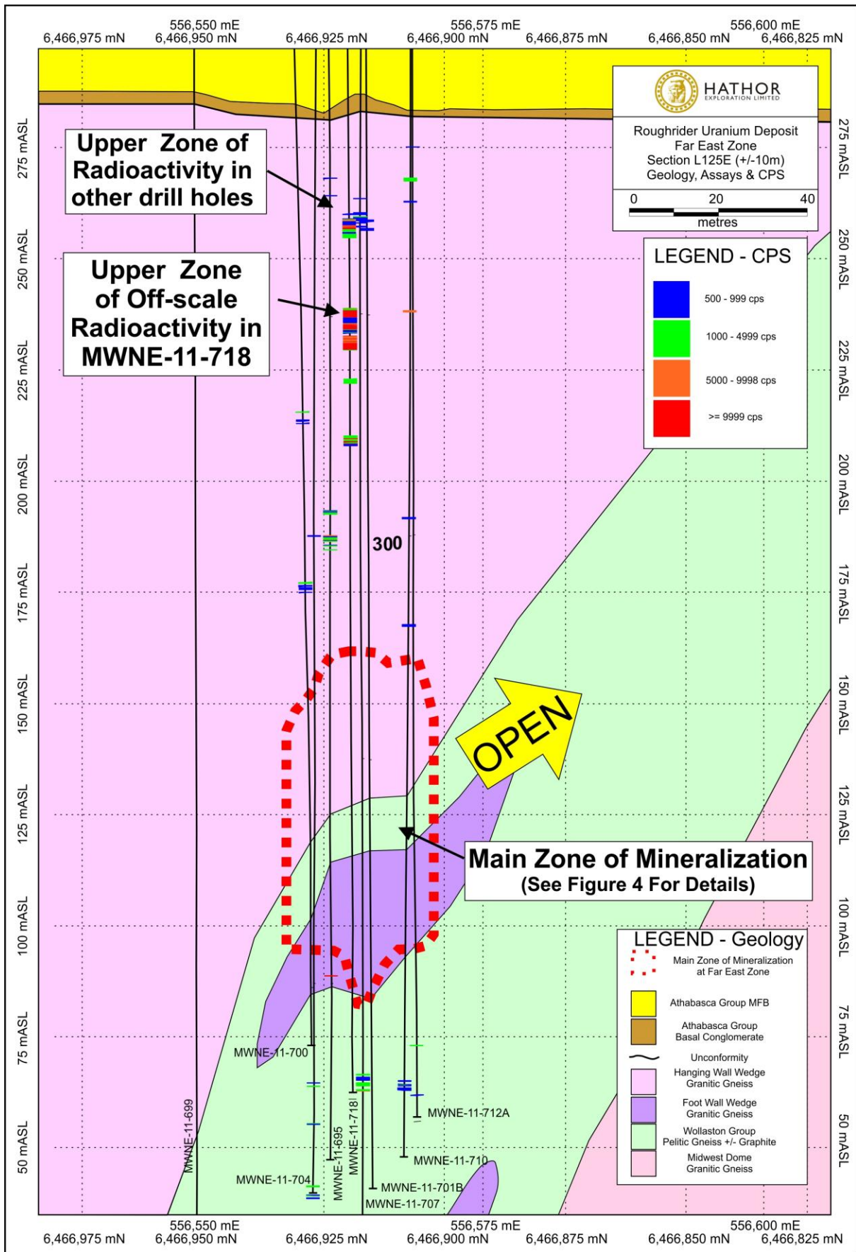
Figure 3: Cross section showing the spatial distribution of the main zone of mineralization and the upper zone of mineralization near the unconformity at Far East Zone at Roughrider; Grid Line 125 East ( \pm 10 m), view northeast. See cross-section in Figure 4 for details of main zone of mineralization.
