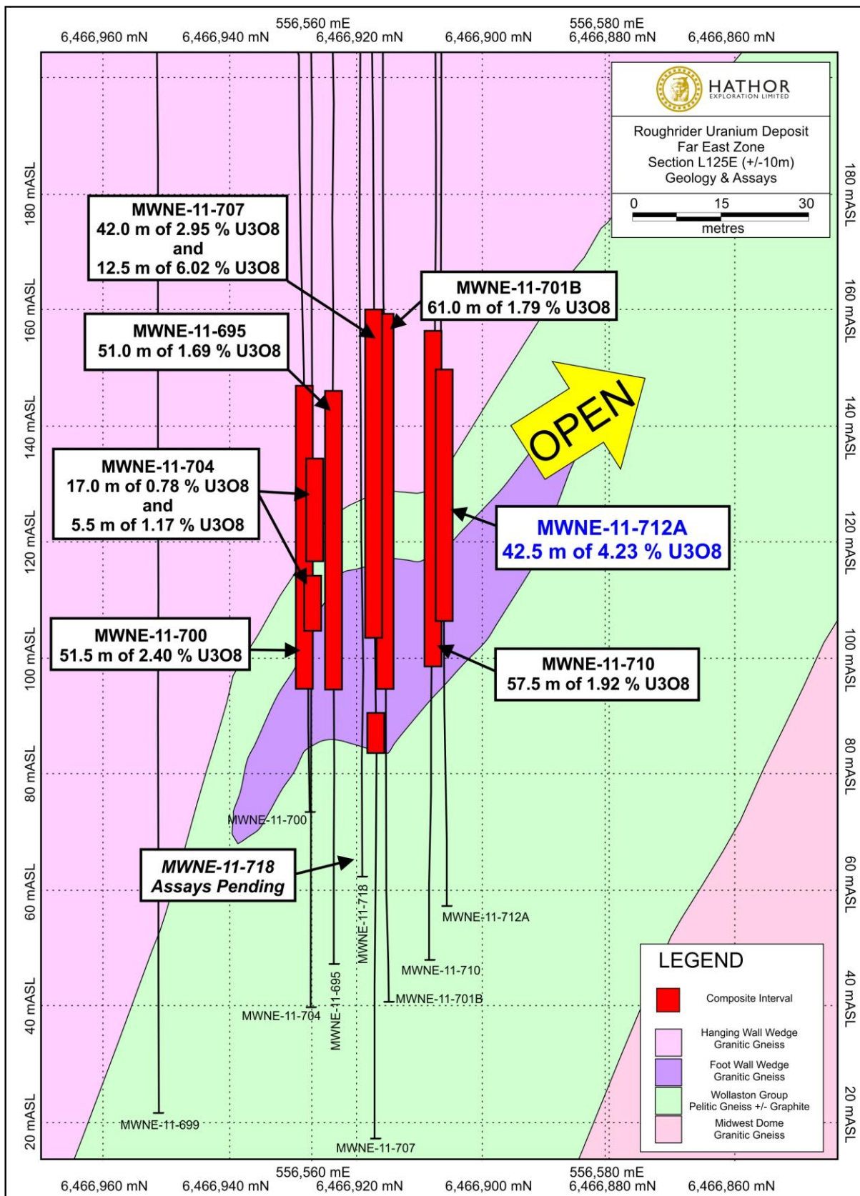
Figure 4: Cross section showing summary composite intervals for the main zone of mineralization at Far East Zone at Roughrider; Grid Line 125 East ( \pm 10 m), view northeast.
