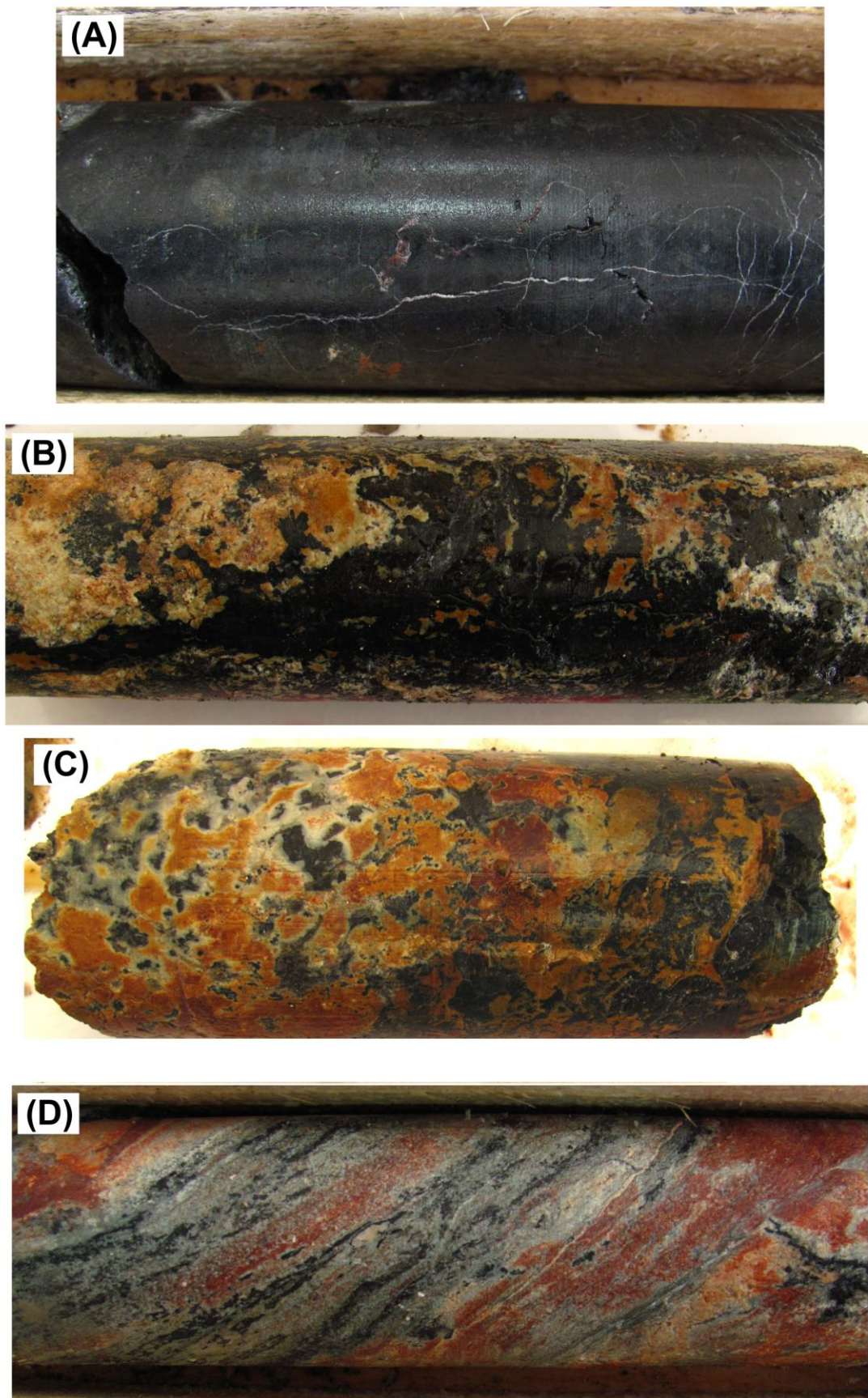
Figure 5: Uranium mineralization styles at Roughrider Far East from drill holes released herein: (A) Massive mineralization, NQ core, MWNE-11-715. (B) Semi-massive mineralization, NQ core, MWNE-11-712A. (C) Hematite-associated mineralization, NQ core, MWNE-11-712A. (D) Foliation parallel mineralization, NQ core, MWNE-11-715.
