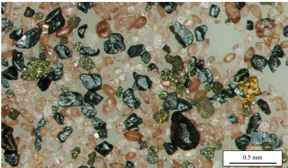
Figure 2: Framboidal pyrite coating gold grains in tailings from wash plant.
