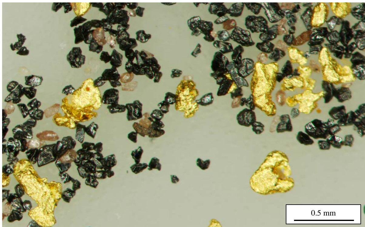
Figure 3: >75 micron gold flakes from primary alluvial deposit at Sourie.
