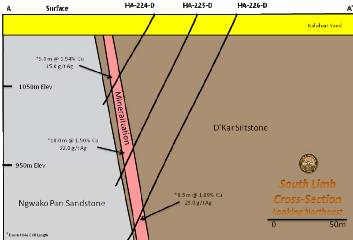
Figure 3: Cross-section through section 64800 (South Limb)
