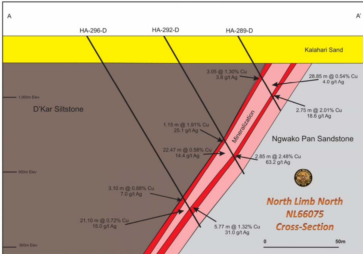
Figure 3: Cross-section through section 66075 (North Limb North)
