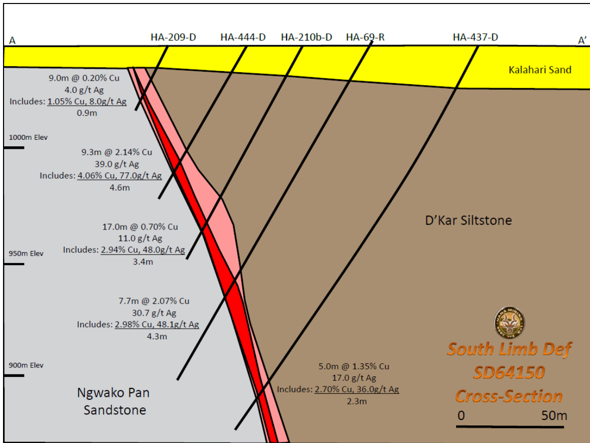
Figure 3: Cross-section through section 64150 (South Limb Definition)
