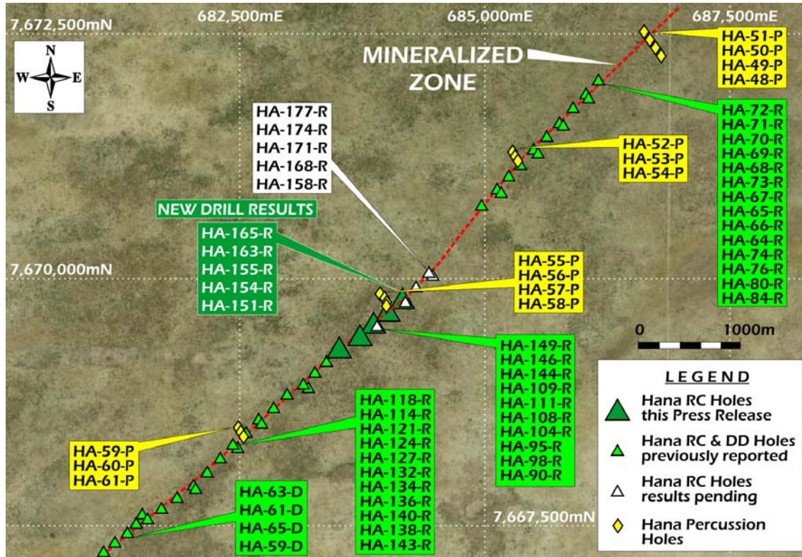
Figure 2: Drill Hole Locations, South Limb (sector 60,000)
