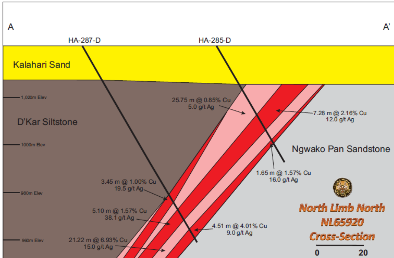
Figure 3: Cross-section through section 65920 (North Limb North)
