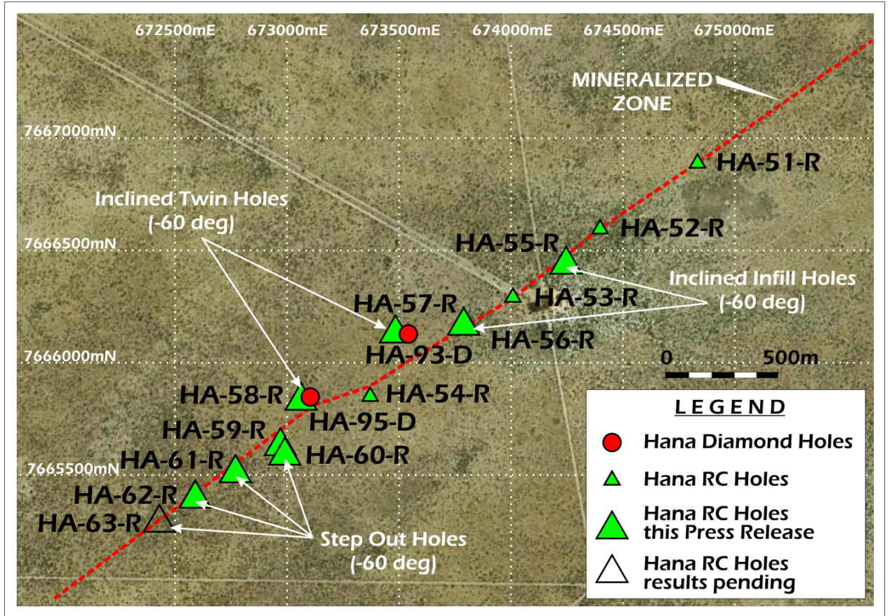
Figure 2: Drill Hole Locations On Western Portion Of North Limb Of Banana Zone (“New Discovery”), Including Both Assayed Holes And Holes Drilled And Awaiting Assay Results
