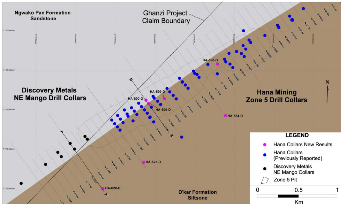
Figure 1: Location of Zone 5 Drilling Results at the Ghanzi Project, Including Sections N123250 to N126750
