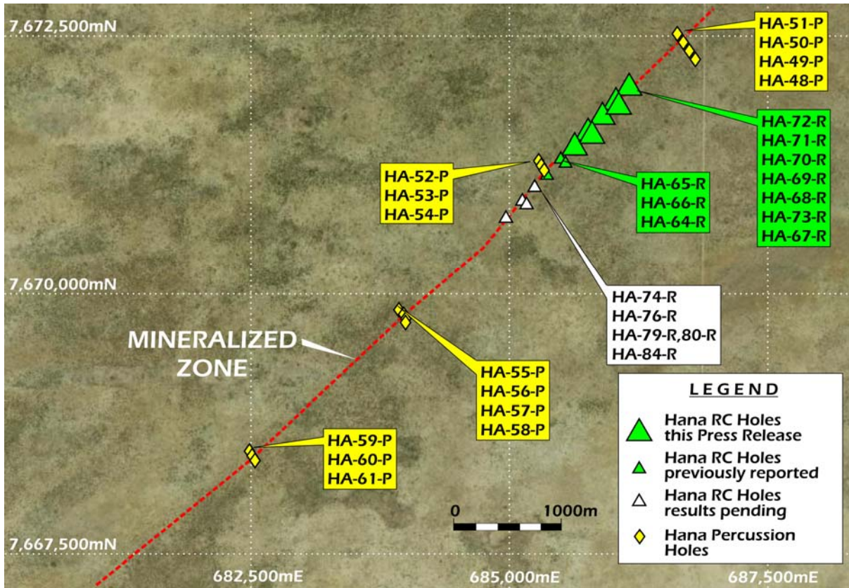
Figure 2: Drill Hole Locations, Northeastern Portion Of South Limb (section 65,000)
