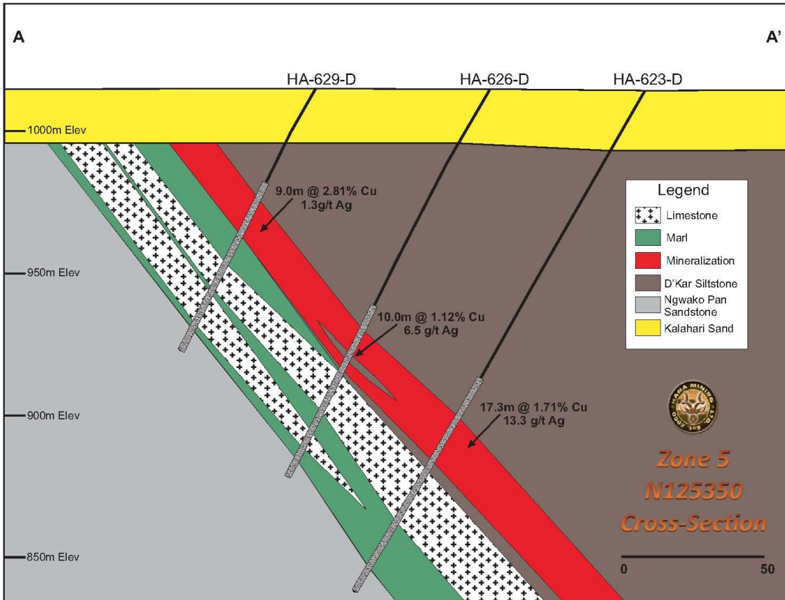
Figure 2: Cross-section through N125350 at Zone 5, showing infill resource drilling; large widths of copper-silver mineralization from three drill collars. High-grade copper mineralization is associated with chalcopyrite, chalcocite and bornite mineralization that occurs as disseminations and/or veinlets found predominately within the siltstone and marl units, but are also commonly found within the carbon rich siltstone and limestone units.
