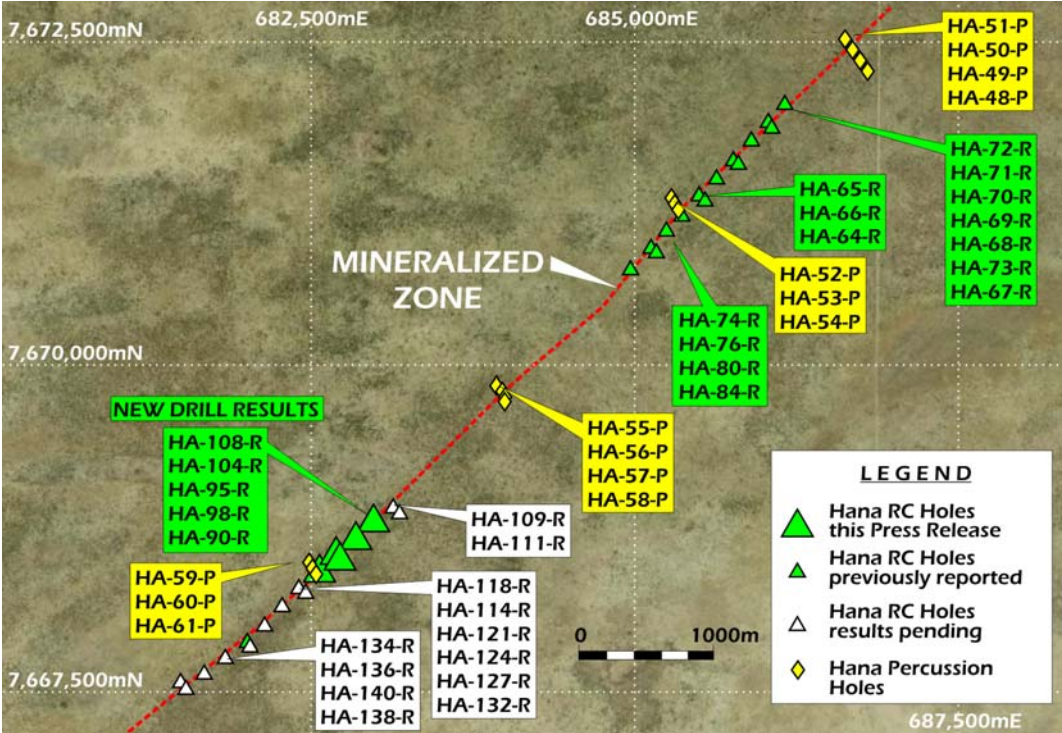
Figure 2: Drill Hole Locations, South Limb (sections 60,000 to 65,000)
