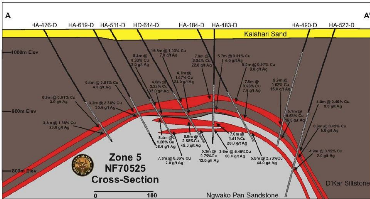
Figure 4: Cross-section of Northeast Fold through section NF70525
