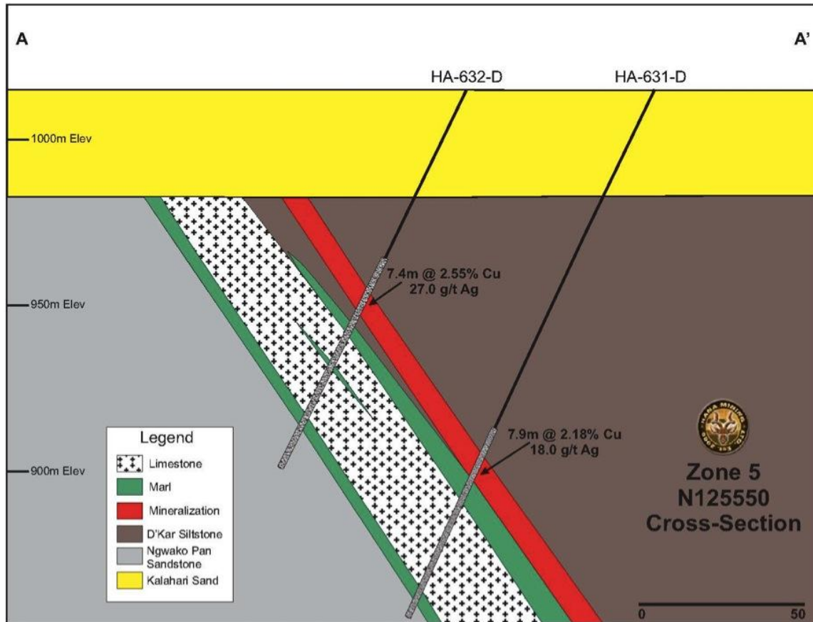
Figure 5: Cross-section through section N125550 (Zone 5)
