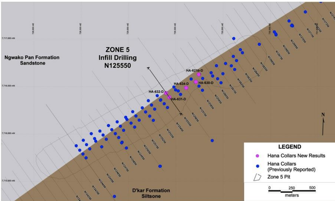
Figure 3: Drill Hole Location of Zone 5, Including Sections HA-621b-D to HA-632-D
