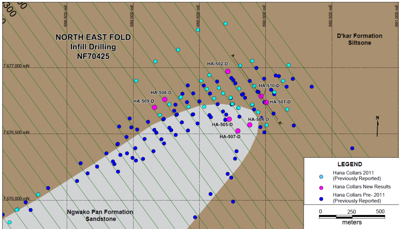
Figure 2: Drill Hole Location of Northeast Fold, Sections 69725-70425
