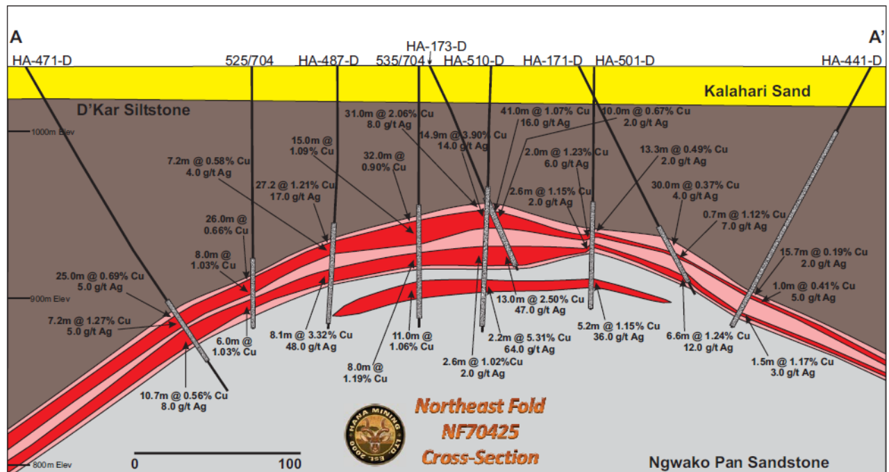
Figure 3: Cross-section through section 70425 (Northeast Fold)
