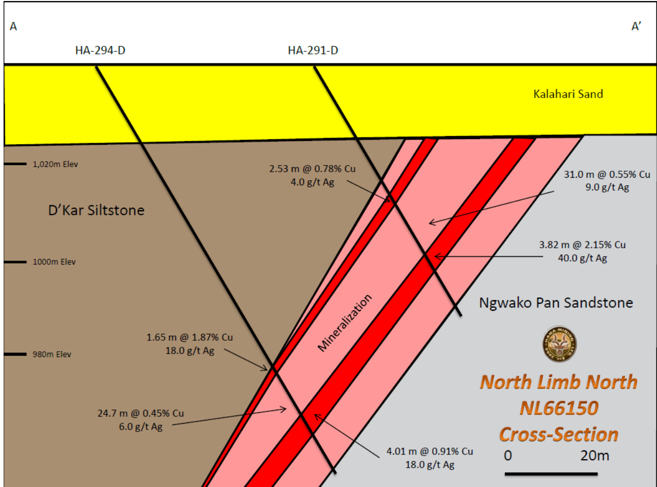
Figure 3: Cross-section through section 66150 (North Limb North)
