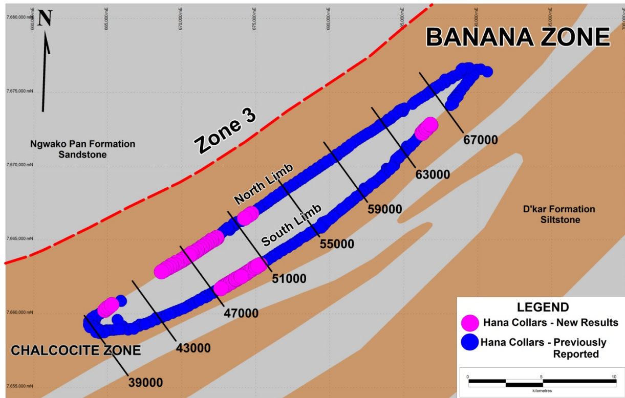
Figure 1: Drill Hole Location – Banana Zone*
