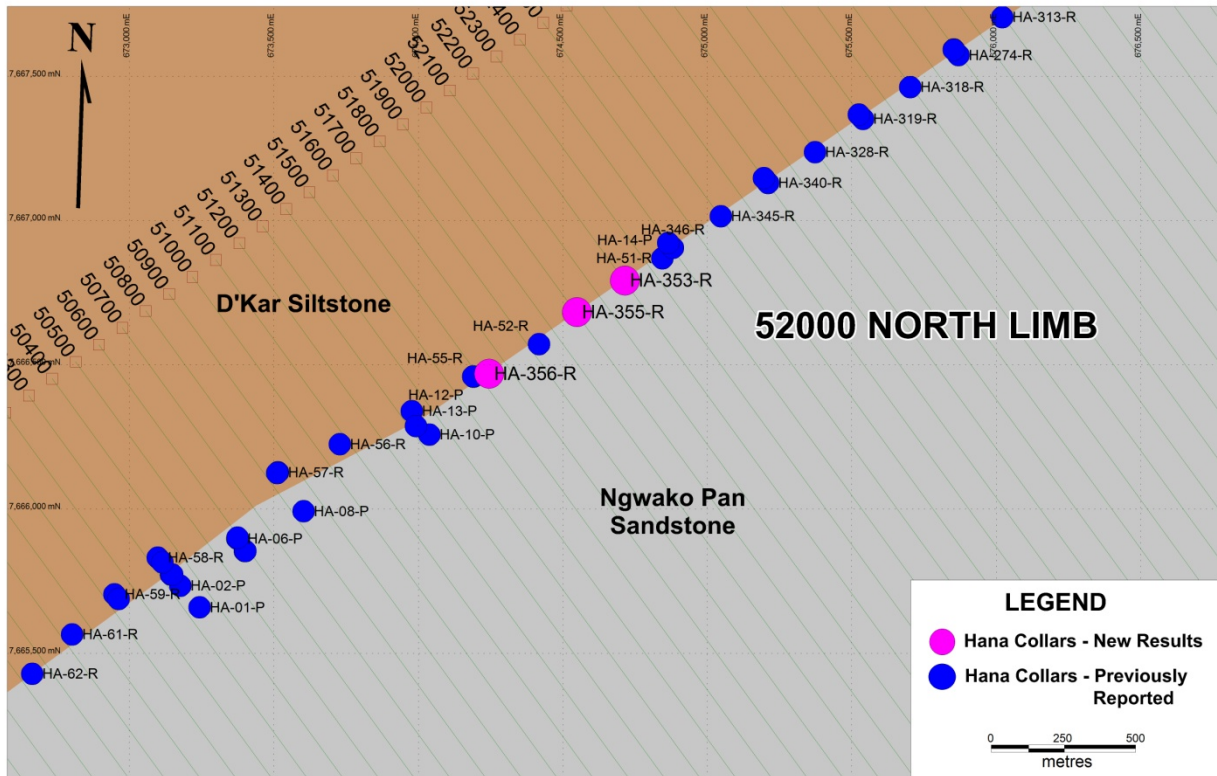
Figure 6: Drill Hole Location of Central North Limb, Section 52000
