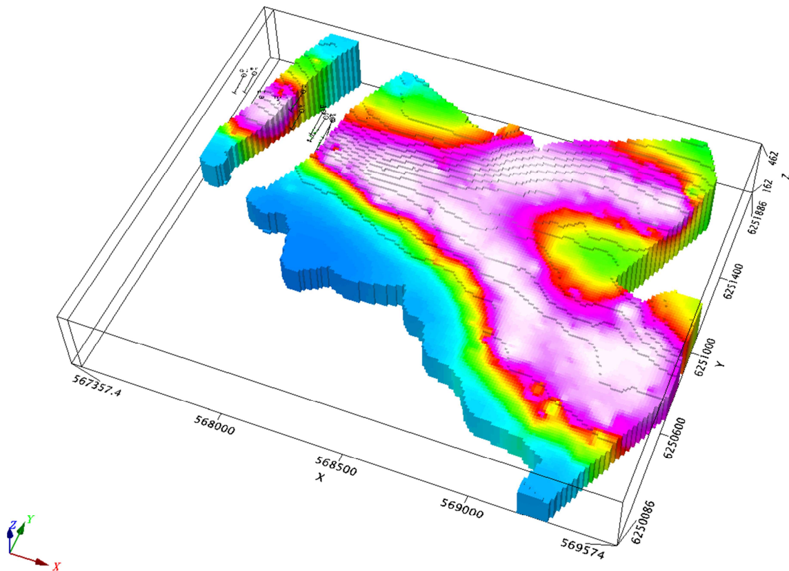
Figure 2 - Resistivity Data at Delhi Pacific
