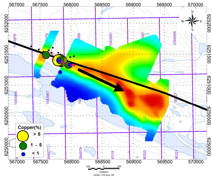
Figure 3 – Resistivity Data at Delhi Pacific
