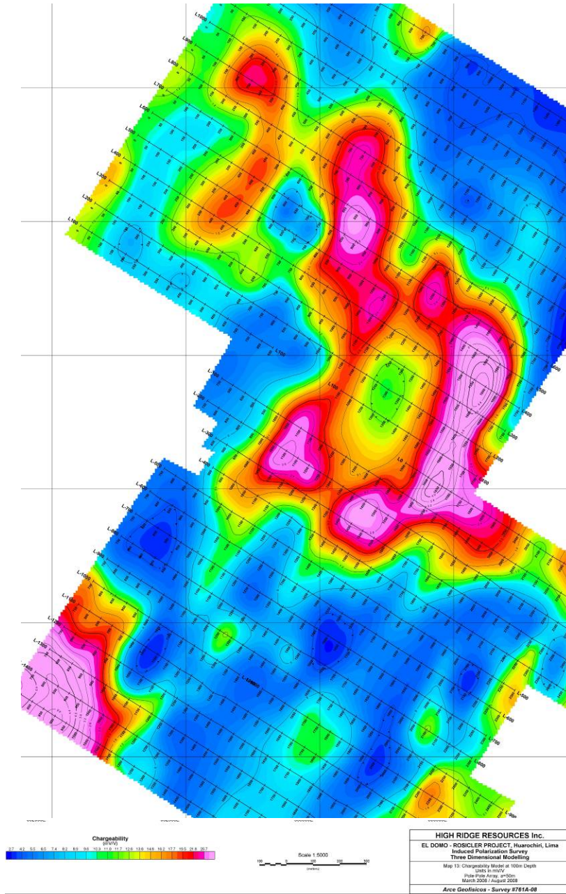
Figure 1. Chargeability model at 100 meters depth for the Rosicler – El Domo project, San Mateo area, Peru.
