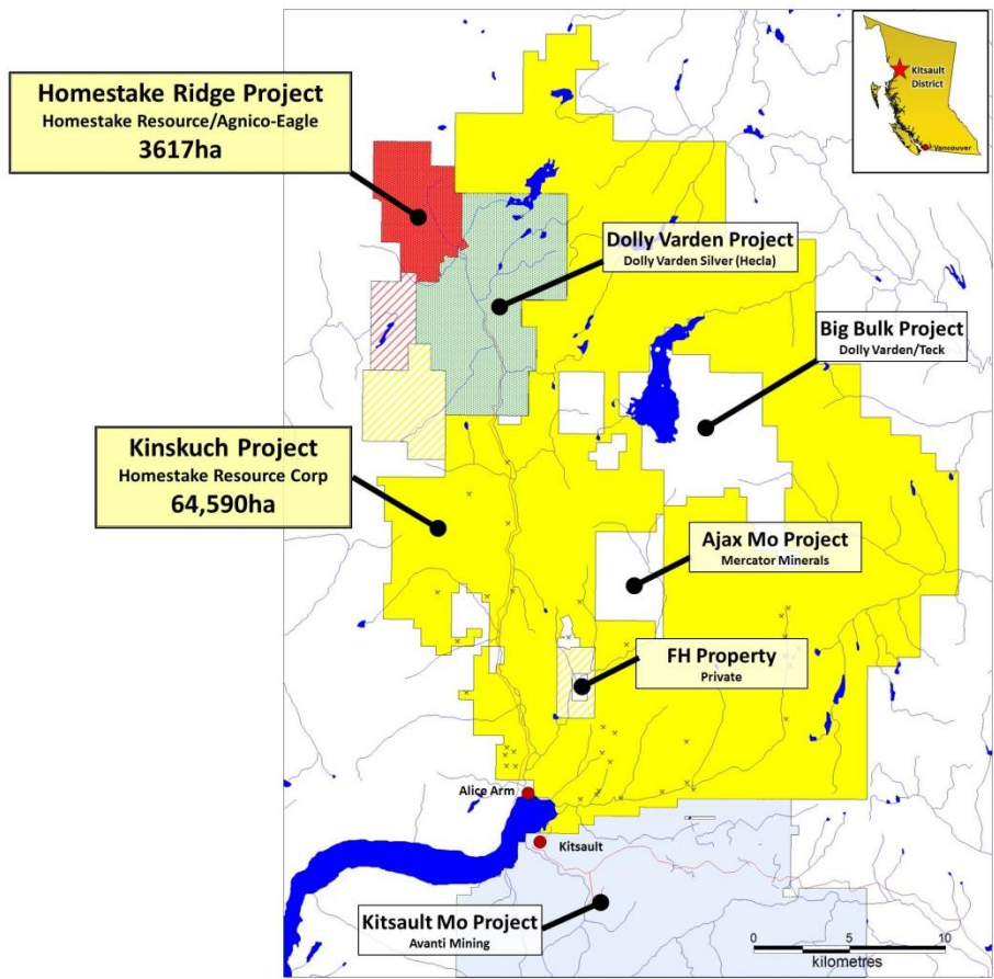
Figure 1: Location of newly staked claims in the Kitsault Mineral District. The hatched patterns show the location of the newly acquired claims for Kinskuch in yellow and Homestake Ridge in red.
