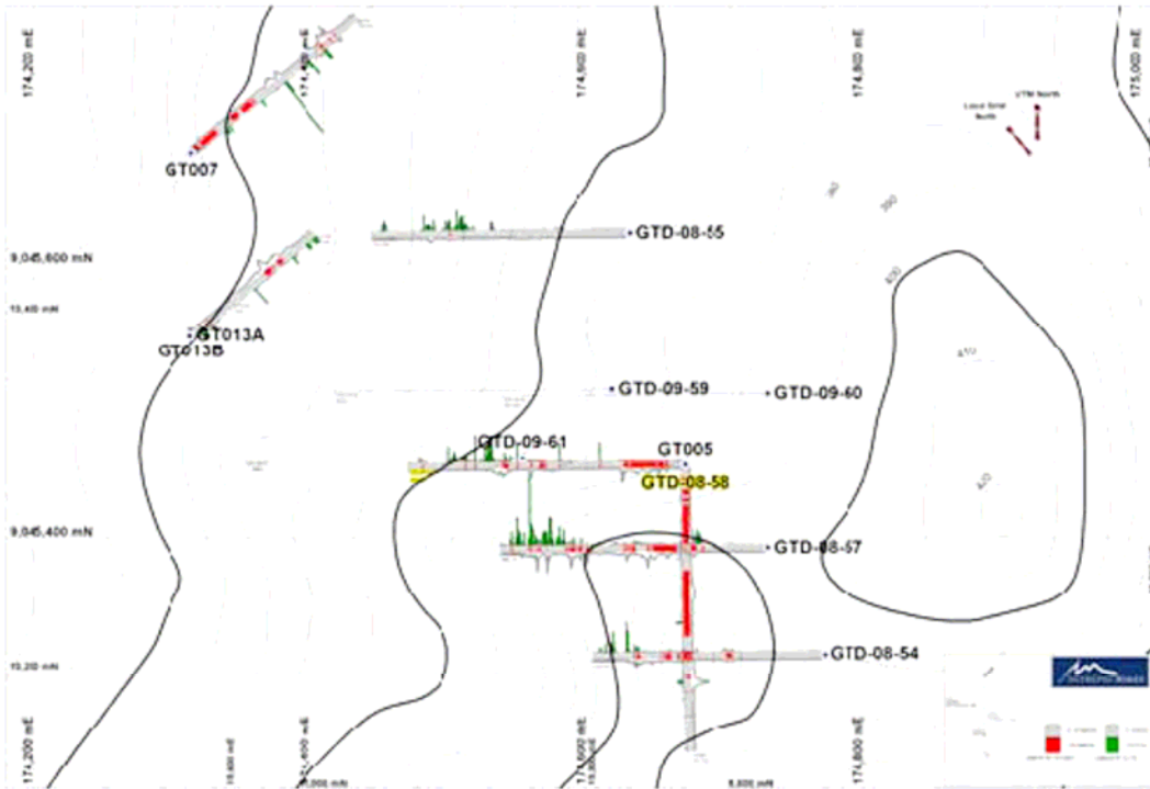
Plan showing location of drill holes in Zone B. Red colouring shows gold intercepts, grey line graph silver, and green histograms copper.
