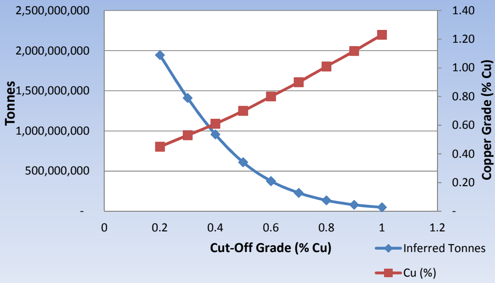
Grade Tonnage Curve - Porphyry Model - Cu% cut-off
